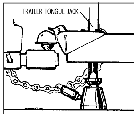
A removable extension helps support the trailer tongue in the trailer ball socket. With the extension removed, the piston has a depression in the top to help center the wheel or bottom of the trailer jack stand.
