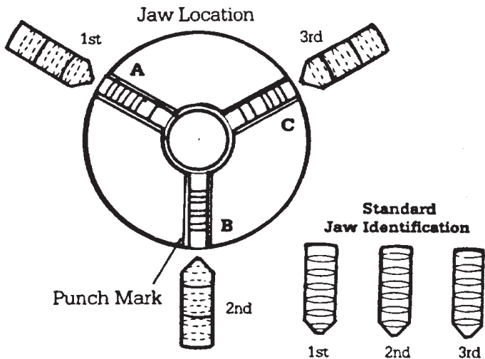
FIGURE 1—Three-Jaw Chuck, standard jaw locations.
