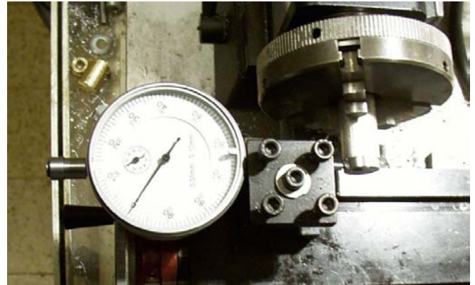
An indicator held in the round hole of the P/N 7600 3/8" tool post is held on the part's centerline.
