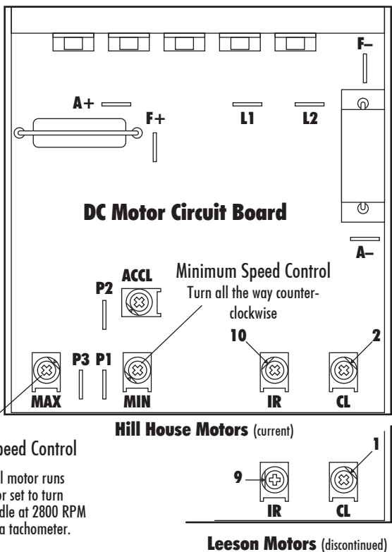
FIGURE 2—Location of terminal connectors and adjustable potentiometers on the speed control circuit board.
