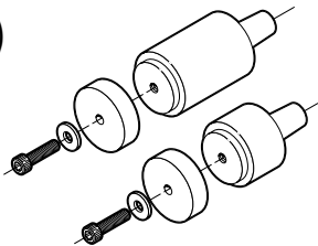
Mill arbor cutters hold 7/8" or 1" I.D. round milling cutters.
