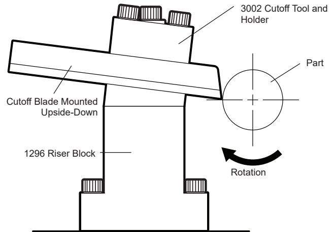
FIGURE 3—Side view of the 3002 cutoff tool holder mounted on top of the P/N 1296 riser with cutting tip pointed downward and adjusted to centerline height. (Seen from headstock spindle.)
