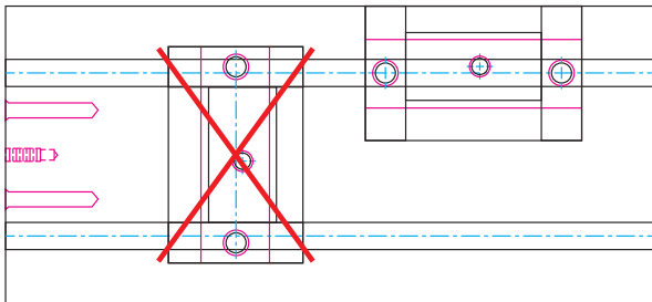
FIGURE 2—Proper mounting orientation on the crossslide.
