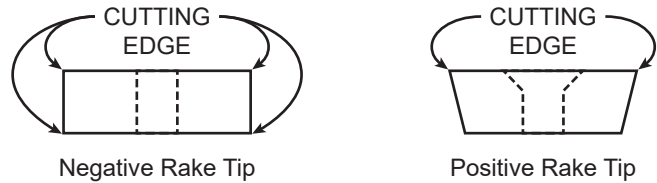
FIGURE 1—Negative and positive rake carbide cutting tips. Negative rake tips can be held upside down giving four cutting edges. Positive rake tips cut from one side only, but cut better.
