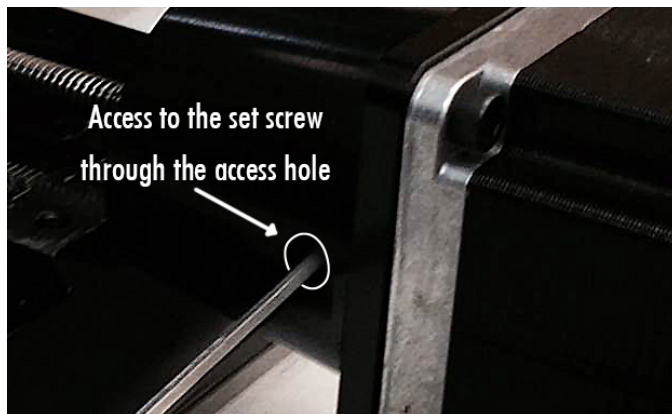
FIGURE 1—Shows the access hole on the motor mount.
